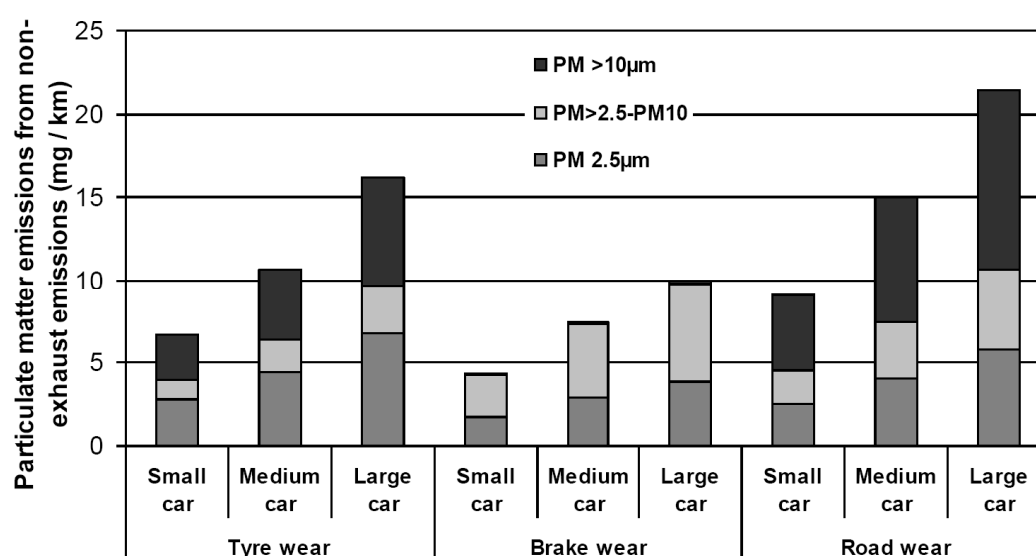
Figure 4. Non-exhaust particulate matter (PM) emissions by source and car size, from Simons [113] based on Ntziachristos and Boulter [117].
